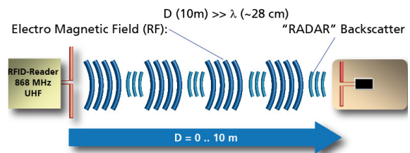
Figure 1: Principle of UHF RFID.
