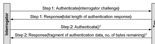
Figure 5: Message exchange for tag authentication.
